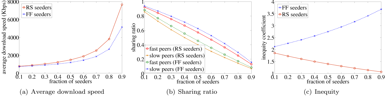
Figure 4: The influence of the seeding strategy: favoring fast peers (FF) or randomly seeding (RS)
