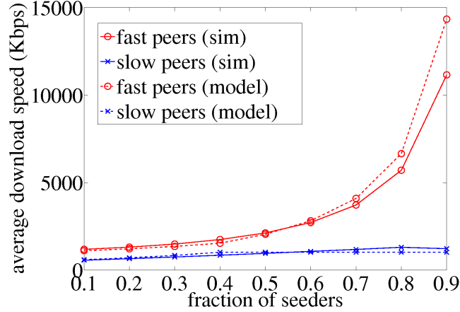
Figure 1: The average download speeds of fast and slow peers in a system with 50 fast peers and 50 slow peers, for different fraction of seeders. The capacities of peers are the following: 1024 Kbps up and \infty down for fast peers; 512 Kbps up and 1024 Kbps down for slow peers. Seeders use the FF policy.
