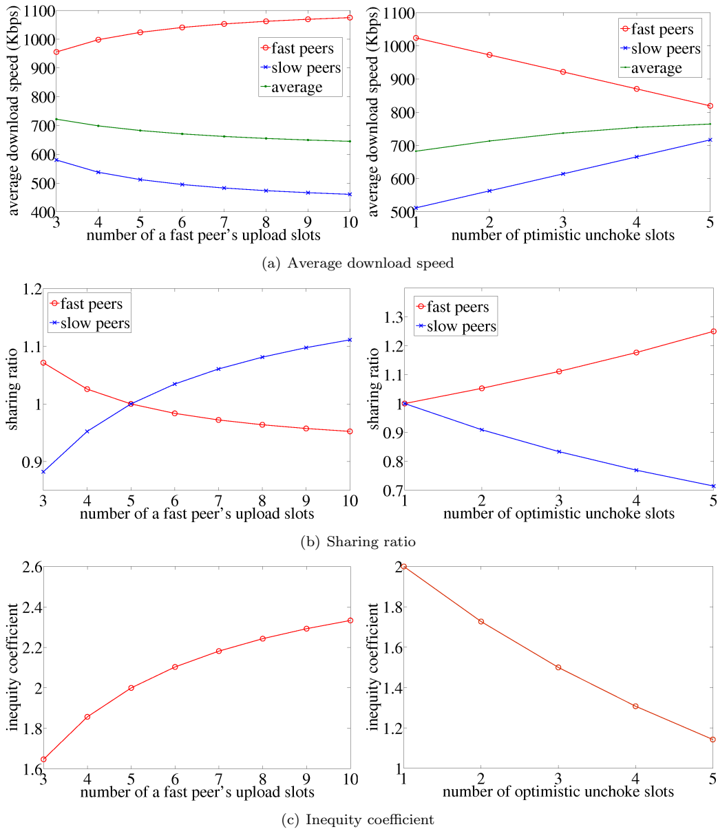
Figure 2: The influence of the number of upload slot in a system with 100 leechers and no seeders.
