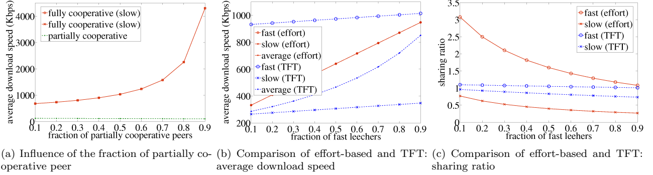
Figure 3: The performance of effort-based mechanism. The fast and slow peer's upload capacities are 1024 and 256 Kbps, respectively.
