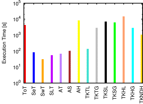
Fig. 6: The query execution times for the 100 GB data set. Logarithmic vertical axis.
