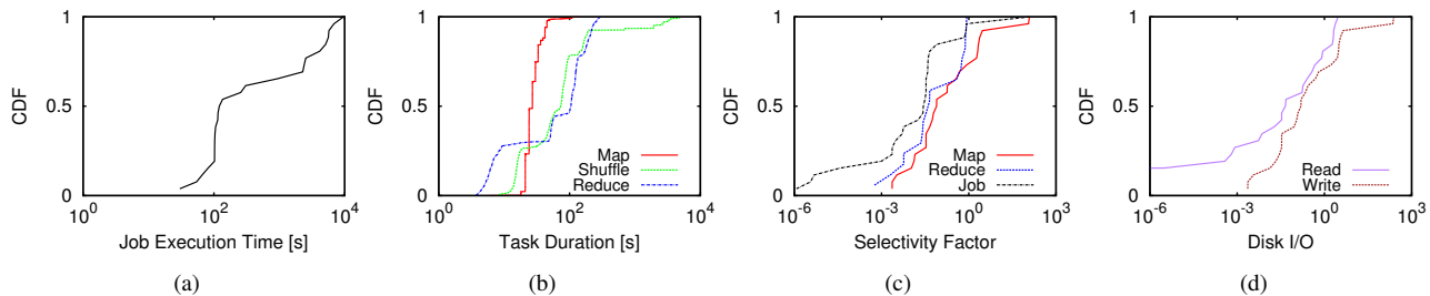
Fig. 7: The MapReduce job profiles: a) the job durations distribution, b) the task durations distribution, c) the task selectivity (ratio between output and input size), and d) the disk I/O (bytes read and written) between tasks, normalized by input size.
