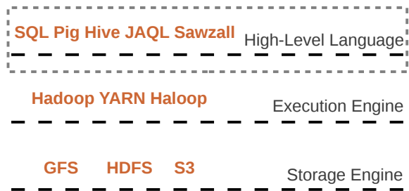
Fig. 2: Our logical workflow occupies the high-level layer of the generic MapReduce software stack for data processing.
