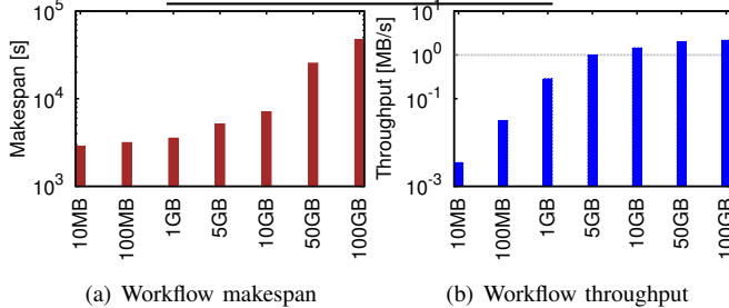
Fig. 4: The makespan and throughput for all input data sizes. The vertical axes are logarithmic and do not start at 1.
