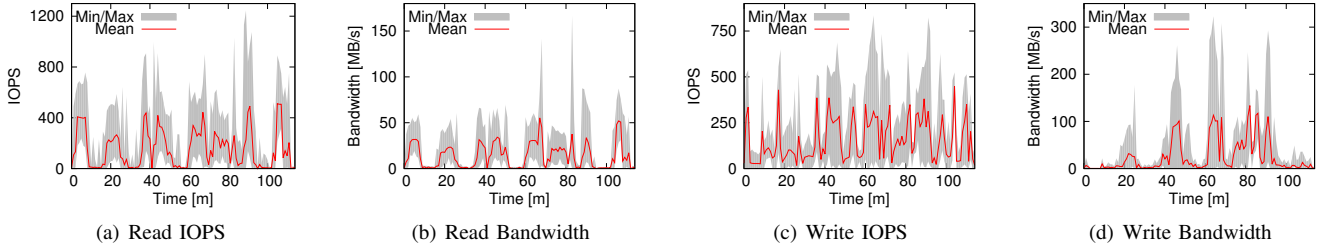
Fig. 5: I/O utilization of the cluster sampled every second and aggregated per minute during the execution of the BTWorld workflow on the 10 GB data set. The gray areas represent the range of observed values.
