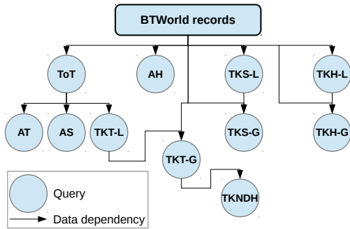
Fig. 3: The BTWorld logical workflow diagram.
