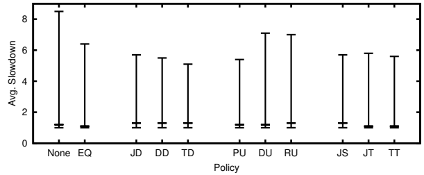
Figure 9: The minimum, the maximum, and the median of the average job slowdowns of 3 MR-clusters with workload WKLD-D for all weighting policies.
