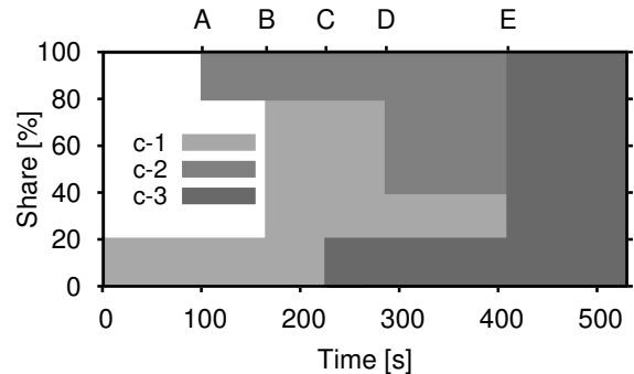
Figure 6: The distribution of the resources across 3 MR-clusters (c-1, c-2, c-3) arriving at different moments in time. (Points A-E explained in Section 7.1.)
